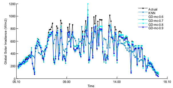
Figure 4. Very short term GSI forecasting based k-NN-learning NN gradient descent and momentum learning algorithm model, actual data, and k-NN method
